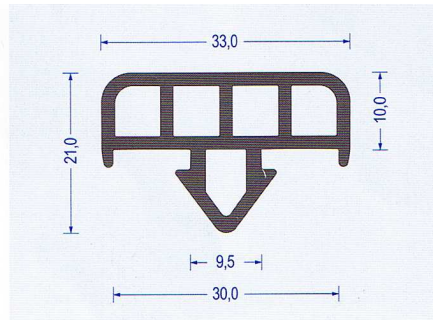
Art.-Nr. 2330005 PVC 70° Shore A schwarz VE : 30 m Bund
