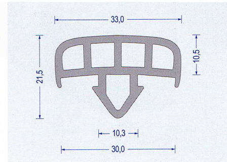
Art.-Nr. 2330006 PvC 85° Shore A grau VE : 30 m Bund
