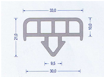
Art.-Nr. 2330004 PVC 70° Shore A grau VE : 30 m Bund
