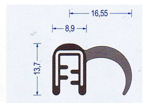
Art.-Nr. 2830010 EPDM schwarz Klemmber. 1-3 mm VE : 50 m Bund Br* a200/b30/c200/d75
