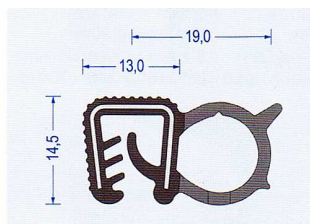
Art.-Nr. 2830013 EPDM schwarz Klemmber. 2-4 mm VE : 75 m Bund Br* a80/b60/c102/d100
