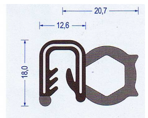
Art.-Nr. 2830018 EPDM schwarz Klemmber. 3-5 mm VE : 50 m Bund Br* a80/b25/c150/d70
