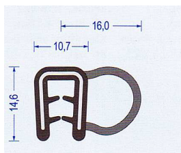
Art.-Nr. 2830011 EPDM schwarz Klemmber. 1,5-3 mm VE : 100 m Bund Br* a40/b30/c180/d40
