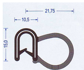
Art.-Nr. 2830015 EPDM schwarz Klemmber. 1-3,5 mm VE : 25 m Bund Br* a200/b80/c200/d200
