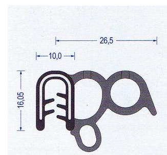
Art.-Nr. 2830031 EPDM schwarz Klemmber. 1,5-3,5 mm VE : 25 m Bund Br* a40/b30/c180/d40
