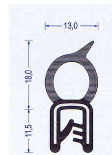
Art.-Nr. 2830028 EPDM schwarz Klemmber. 1-2,5 mm VE : 50 m Bund Br* a100/b180/c25/d25
