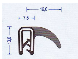
Art.-Nr. 2830007 EPDM schwarz Klemmber. 1-2 mm VE : 50 m Bund Br* a80/b40/c200/d200
