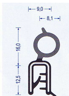
Art.-Nr. 2830026 EPDM schwarz Klemmber. 1-2,5 mm VE : 100 m Bund Br* a100/b200/c100/d60
