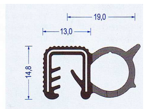
Art.-Nr. 2830014 EPDM schwarz Klemmber. 4-6 mm VE : 75 m Bund Br* a80/b60/c120/d100
