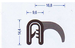
Art.-Nr. 2830008 EPDM schwarz Klemmber. 1-2,5 mm VE : 100 m Bund Br* a80/b120/c-d-
