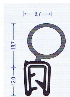
Art.-Nr. 2830027 EPDM schwarz Klemmber. 1-3 mm VE : 50 m Bund Br* a160/b250/c200/d-
