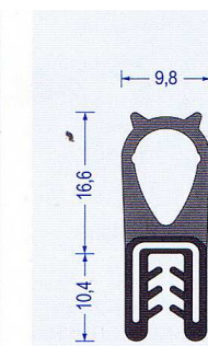
Art.-Nr. 2830030 EPDM schwarz Klemmber. 1-3 mm VE : 50 m Bund Br* a80/b150/c20/d20
