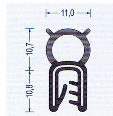
Art.-Nr. 2830023 EPDM schwarz Klemmber. 1-3 mm VE : 50 m Bund Br* a50/b180/c30/d30
