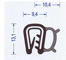
Art.-Nr. 2830006 EPDM schwarz Klemmber. 2 mm VE : 50 m Bund Br* a30/b40/c30/d60
