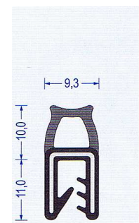
Art.-Nr. 2830025 EPDM schwarz Klemmber. 1-3 mm VE : 50 m Bund Br* a60/b200/c25/d25
