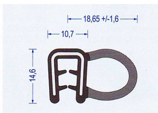
Art.-Nr. 2830012 EPDM schwarz Klemmber. 1,5-3 mm VE : 25 m Bund Br* a80/b60/c200/d80
