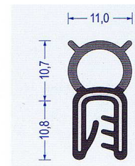
Art.-Nr. 2830024 NBR schwarz Klemmber. 1-3 mm VE : 50 m Bund Br* a50/b180/c30/d30
