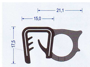
Art.-Nr. 2830017 EPDM schwarz Klemmber. 5-9 mm VE : 50 m Bund Br* a80/b60/c-d-
