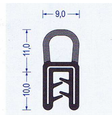
Art.-Nr. 2830022 EPDM schwarz Klemmber. 1-2,5 mm VE : 100 m Bund Br* a60/b120/c25/d25
