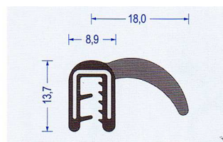
Art.-Nr. 2830009 EPDM schwarz Klemmber. 2-3 mm VE : 50 m Bund Br* a45/b10/c75/d250
